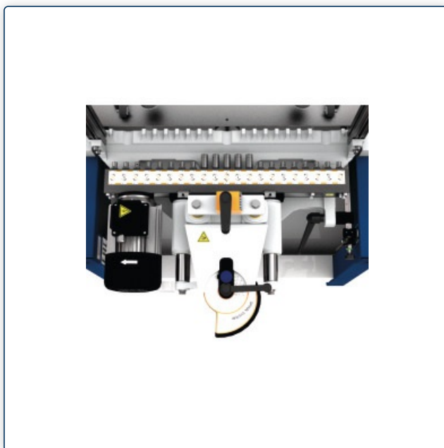
Patented system for quick and easy drilling depth adjustment via spiral disc
