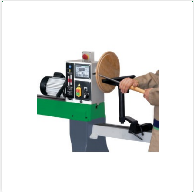
The headstock can be pivoted for turning workpieces in cross grain operations that are larger than the inside dimension of the Lathe. The optional bed extension in combination with the convertible manual tool support ensure maximum flexibility.
