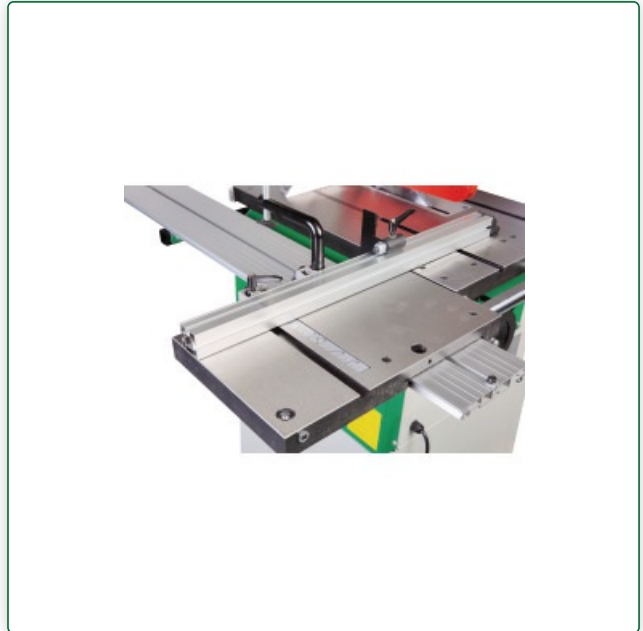
Saw blade pivoting from 90 ° to -45 ° to the left
