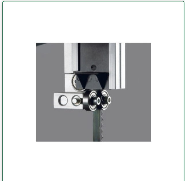
Low-friction, precise and easily adjustable 3-roller saw band guide on top.
