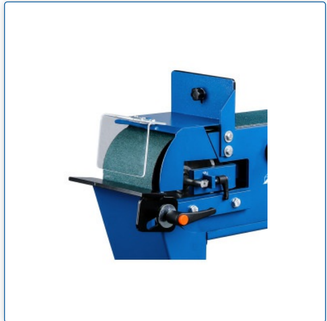
Easy adjustment of the belt run using the adjusting screw
